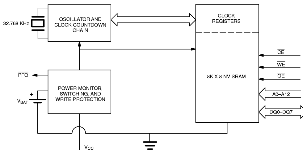
DS1643 BLOCK DIAGRAM Figure 1
